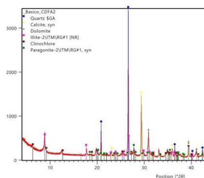
Figura 2. Diffractograma CDFA2
