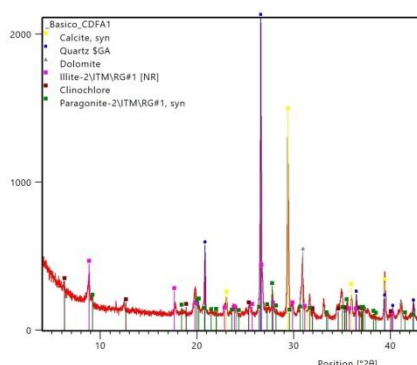
Figura 1. Diffractograma CDFA1
