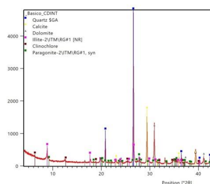
Figura 3. Diffractograma CDINT
